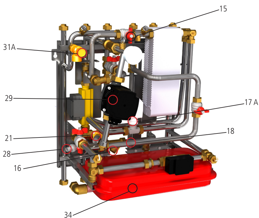
System 5 Split
