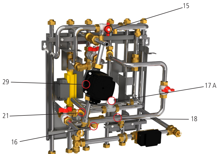
System 3 Split
